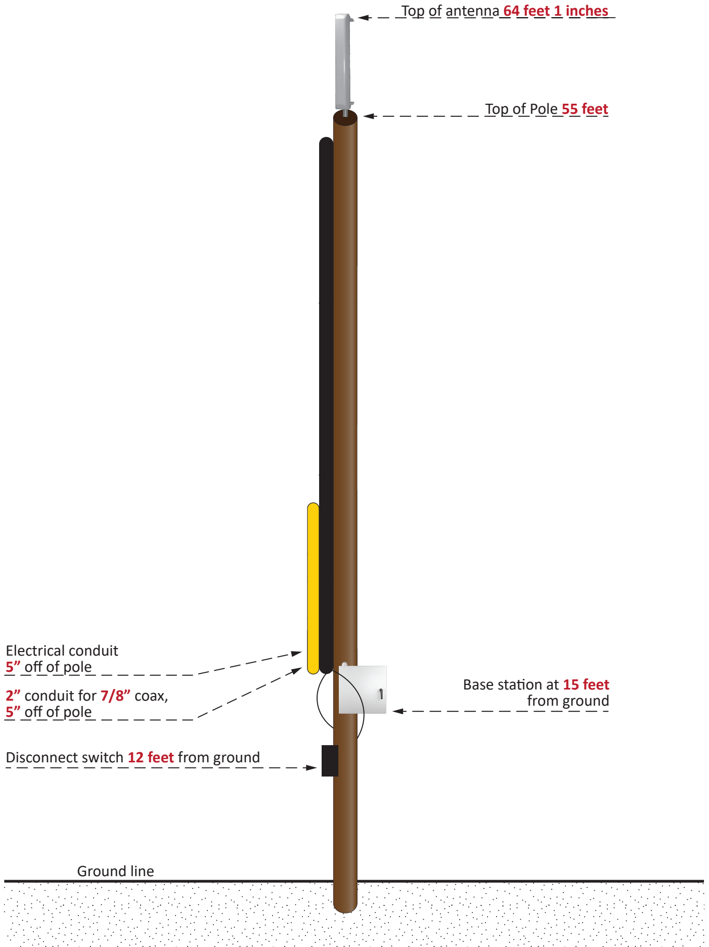
FIGURE 2: POLE DIAGRAM
